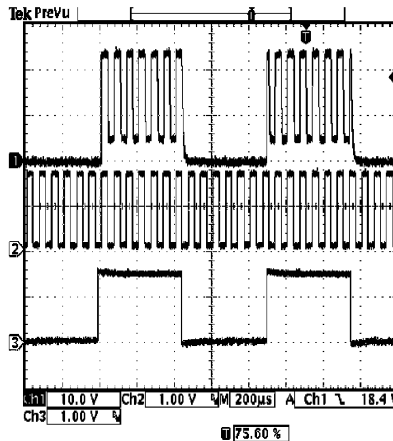
Figure 46. Waveform
