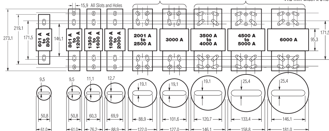
Figure 28.0-25. Typical Fuse Dimensions in Millimeters
