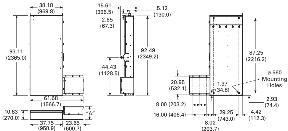
Figure 28.0-16. Quick-Connect Double-Throw 600–800A—Dimensions in Inches (mm)
