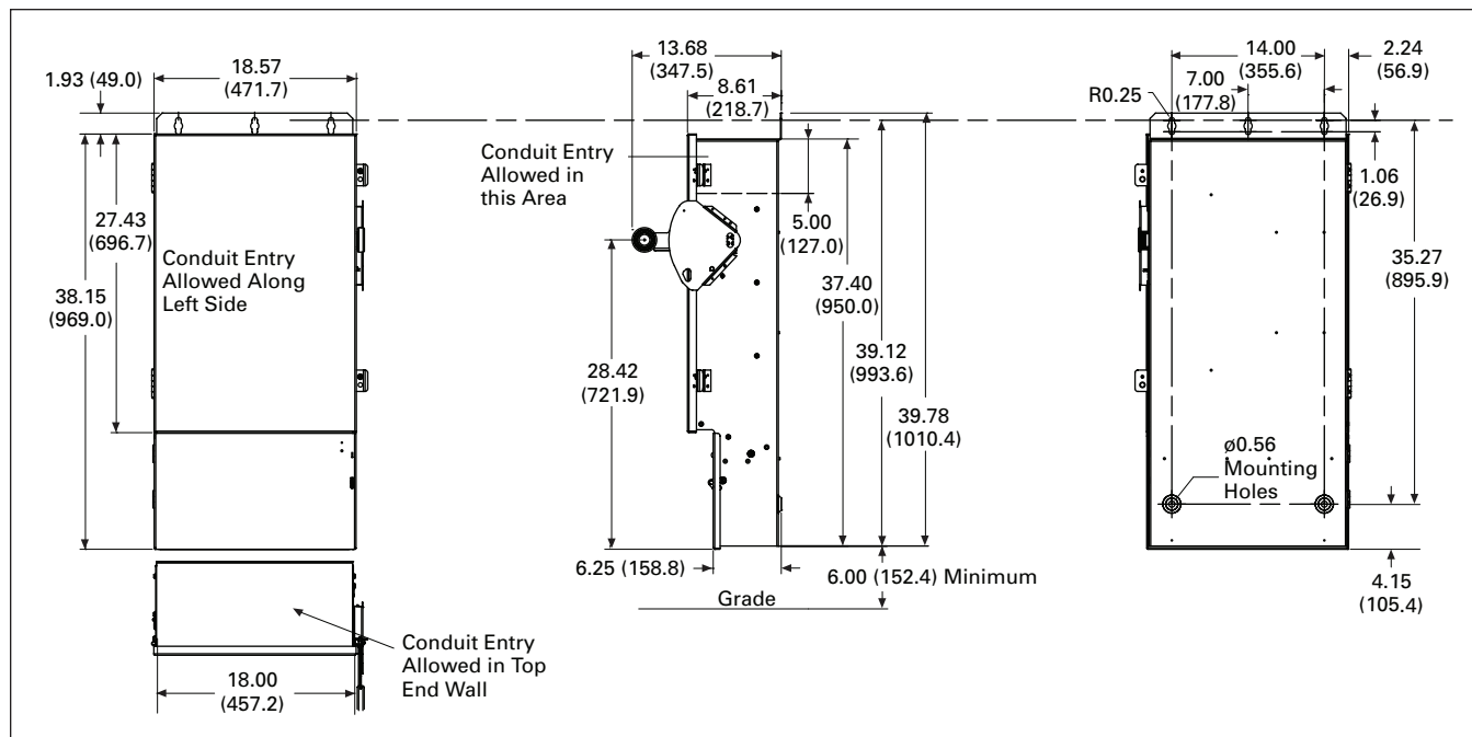
Figure 28.0-17. Quick-Connect Single-Throw 100A—Dimensions in Inches (mm)
