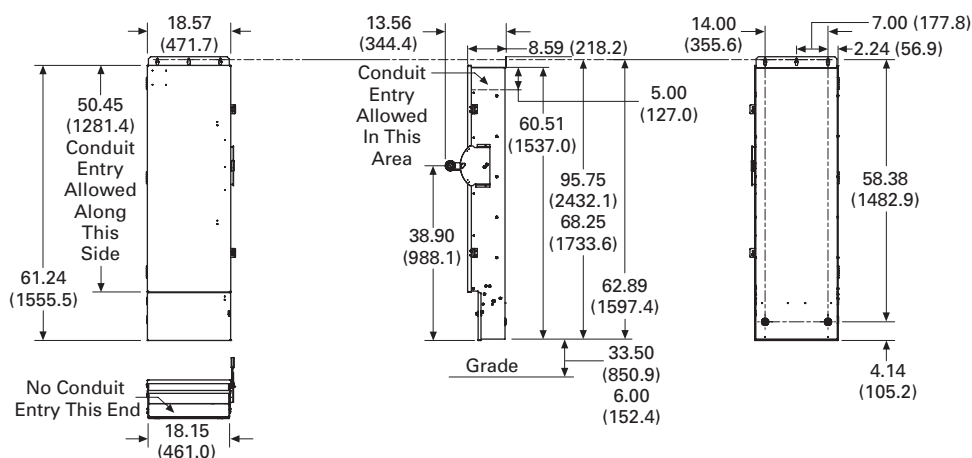
Figure 28.0-14. Quick-Connect Double-Throw 30/200A—Dimensions in Inches (mm)
