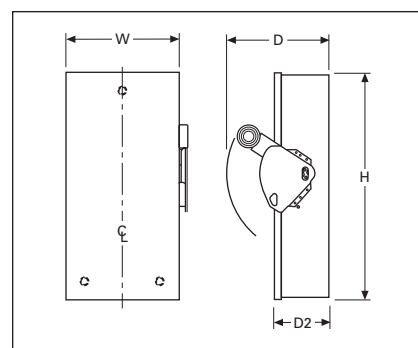
Figure 28.0-10. NEMA 1, 3R 30-1200A
