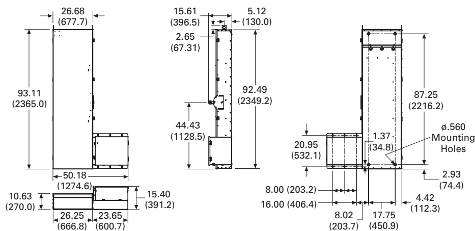
Figure 28.0-15. Quick-Connect Double-Throw 400A—Dimensions in Inches (mm)
