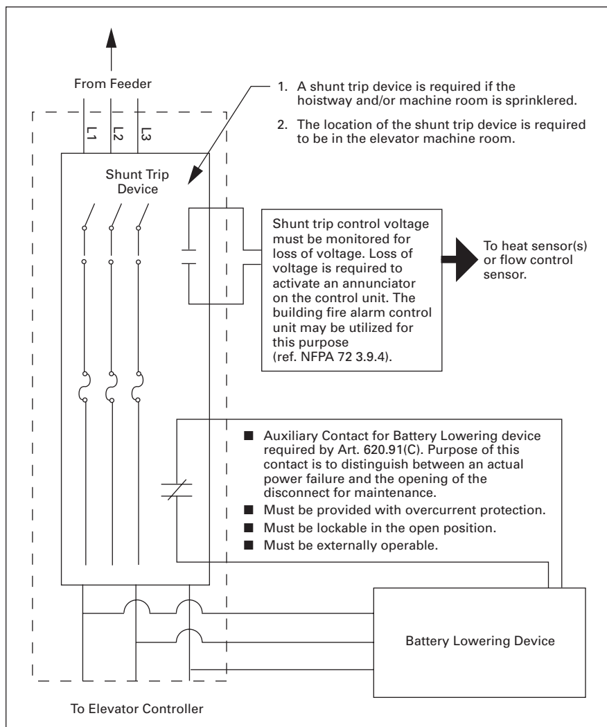
Figure 28.0-3. Shunt Trip Device Wiring Diagram
