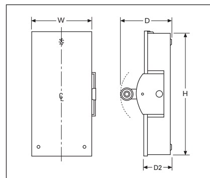
Figure 28.0-12. NEMA 1, 3R 30-800A
