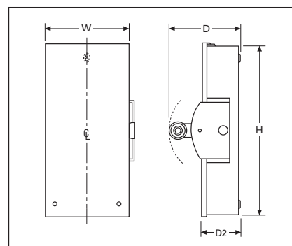
Figure 28.0-8. NEMA 1, 3R 30-800A
