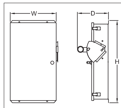
Figure 28.0-22. Elevator Control Switch Diagram
