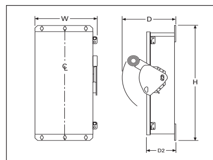
Figure 28.0-7. NEMA 4/4X and 12 30-800A
