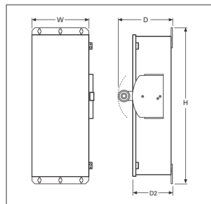
Figure 28.0-13. NEMA 12, 4X 30-400A
