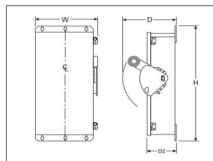
Figure 28.0-11. NEMA 4/4X and 12 30-800A
