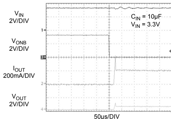
Figure 15. Current Limit Response Time (Output is loaded by 2.2Ω, C_{OUT} = 0.1\mu F )
