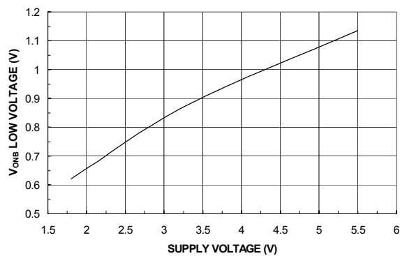
Figure 4. VONB Low Voltage vs. Input Voltage
