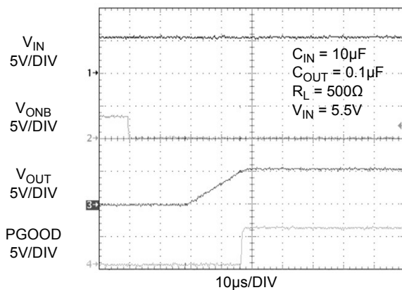
Figure 17. PGOOD Response
