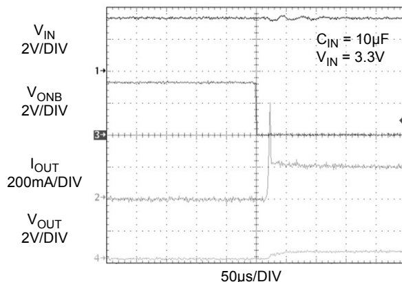
Figure 16. Current Limit Response Time (Output is loaded by 2.2Ω, C_{OUT} = 10\mu F )
