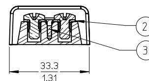
SECTION Z-Z
