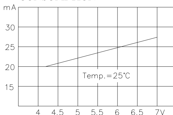
VOLTAGE-CURRENT CONSUMPTION
