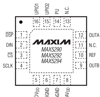
(4mm x 4mm) THIN QFN
