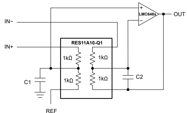
Unity-Gain Difference Amplifier
