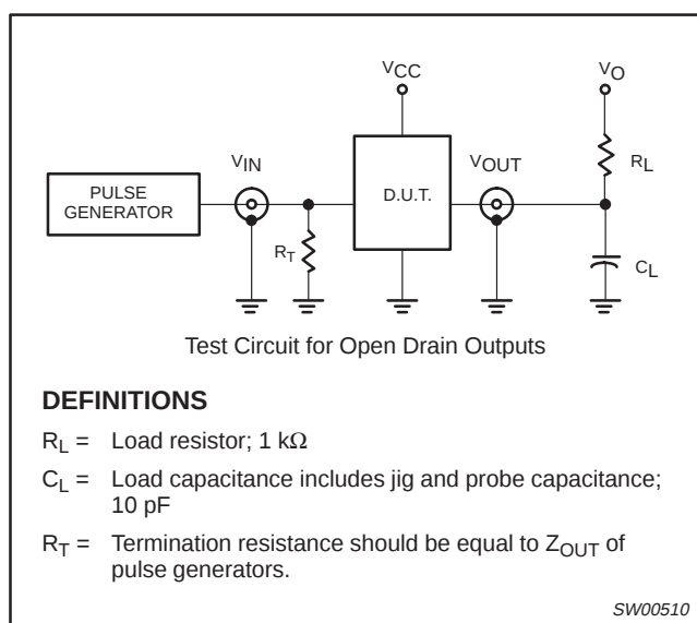
Figure 14. Test circuit
