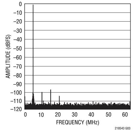
LTC2185: 64k Point FFT, f_{IN} = 5\text{MHz} , -1\text{dBFS} , 125Msps
