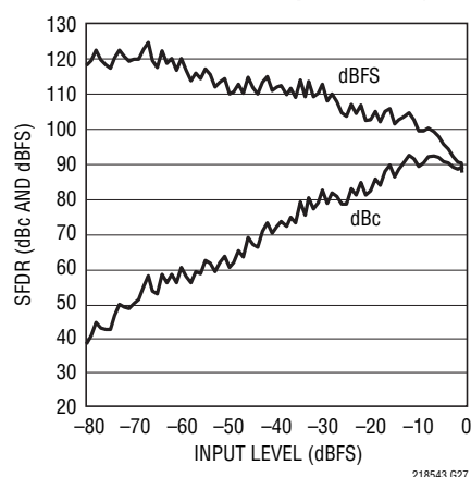
LTC2183: SFDR vs Input Level, f_{IN} = 70\text{MHz} , 80\text{Mps} , 2\text{V} Range
