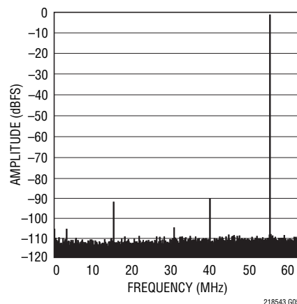
LTC2185: 64k Point FFT, f_{IN} = 70\text{MHz} , -1\text{dBFS} , 125Msps
