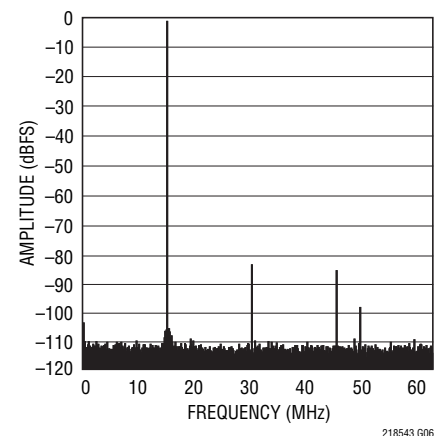
LTC2185: 64k Point FFT, f_{IN} = 140\text{MHz} , -1\text{dBFS} , 125Msps
