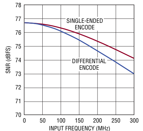
LTC2184: SNR vs Input Frequency, -1\text{dBFS} , 105Mps, 2V Range
