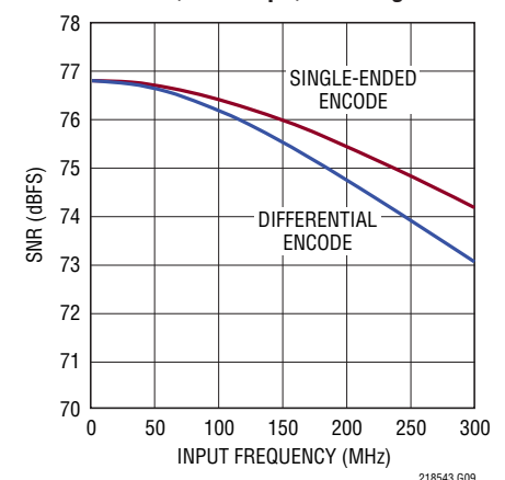
LTC2185: SNR vs Input Frequency, -1\text{dBFS} , 125Msps, 2V Range
