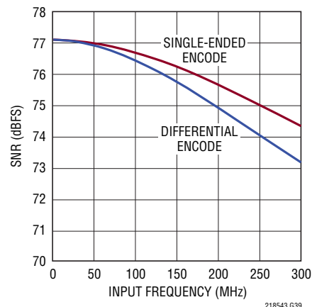
LTC2183: SNR vs Input Frequency, -1\text{dBFS} , 80\text{Mps} , 2\text{V} Range
