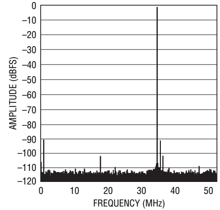
LTC2184: 64k Point FFT, f_{IN} = 140\text{MHz} , -1\text{dBFS} , 105Mps
