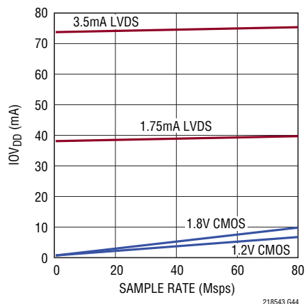
LTC2183: I_{OVD} vs Sample Rate, 5\text{MHz} , -1\text{dBFS} Sine Wave Input on Each Channel
