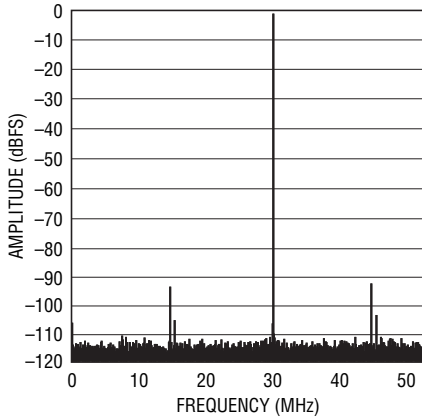
LTC2184: 64k Point FFT, f_{IN} = 30\text{MHz} , -1\text{dBFS} , 105Mps
