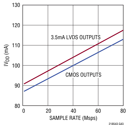
LTC2183: I_{VDD} vs Sample Rate, 5\text{MHz} , -1\text{dBFS} Sine Wave Input on Each Channel
