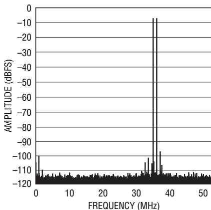
LTC2184: 64k Point 2-Tone FFT, f_{IN} = 69\text{MHz} , 70\text{MHz} , -7\text{dBFS} , 105Mps
