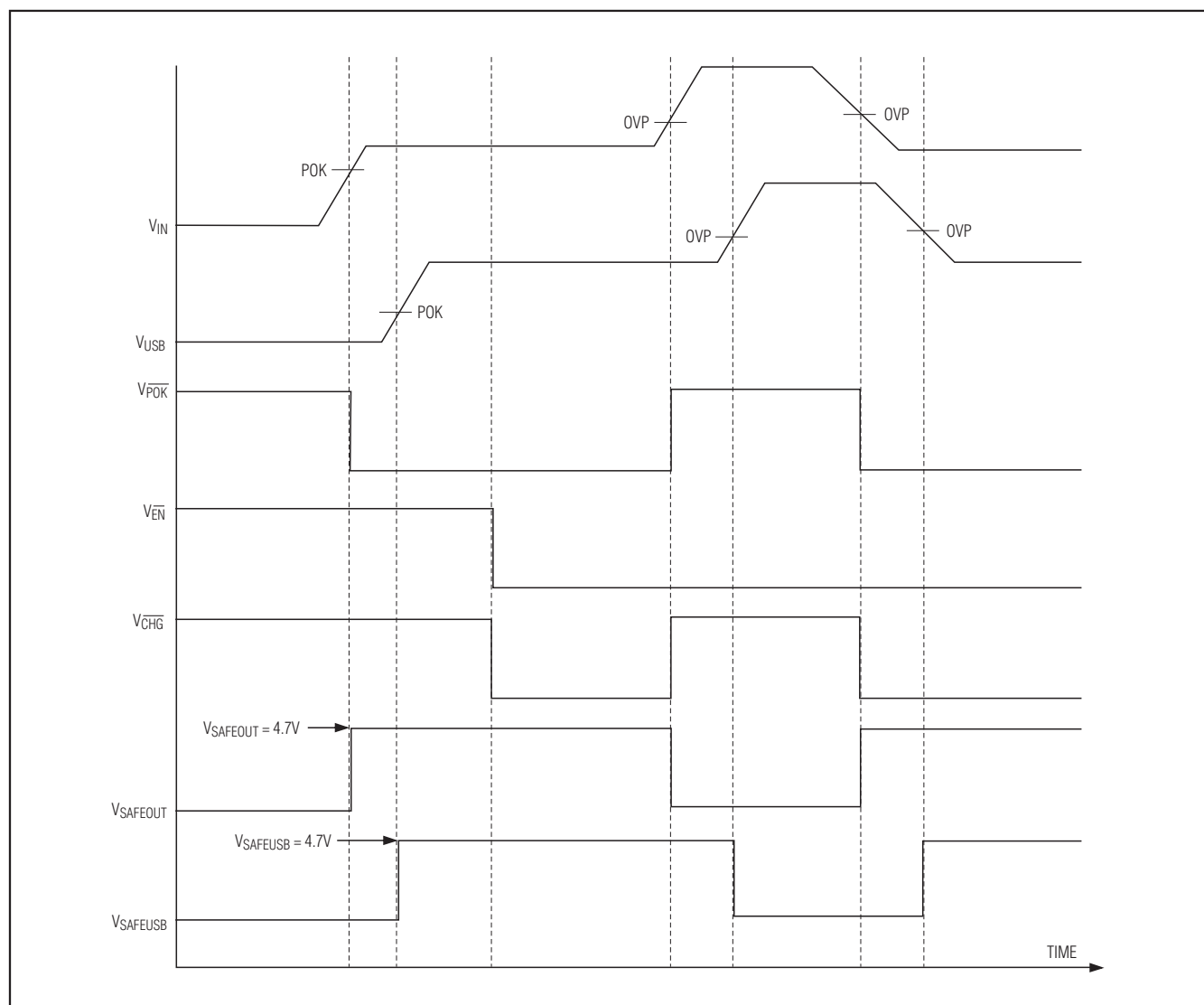
Figure 7. Timing Diagram
