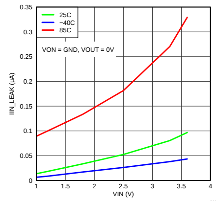
Figure 2. V_{IN} vs. I_{IN(LEAK)}
