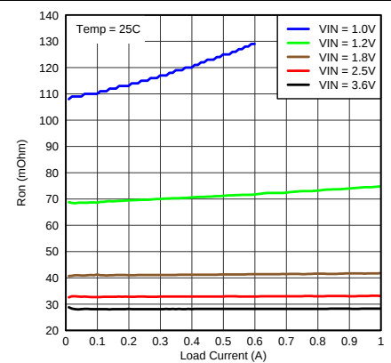
Figure 6. R_{ON} vs. Load Current (Various V_{IN} at T_A = 25^\circ C )
