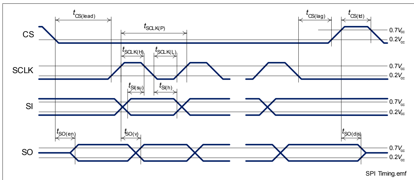
Figure 12 Timing Diagram
