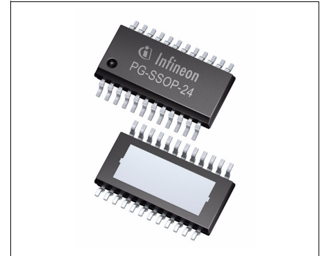
PG-SSOP-24-4
