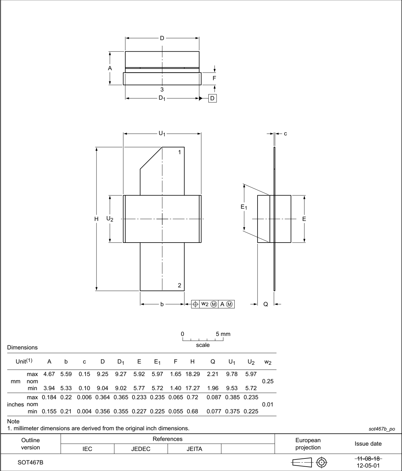
Fig 15. Package outline SOT467B
