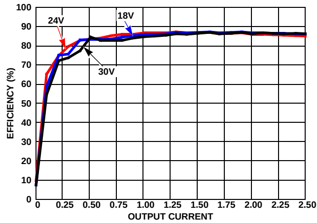
FIGURE 1. EFFICIENCY PLOTS
