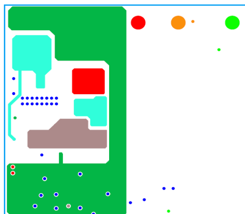
FIGURE 21. ETCH - LAYER 3
