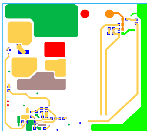
FIGURE 22. ETCH - BOTTOM LAYER
