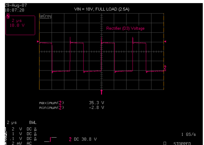
FIGURE 9. RECTIFIER WAVEFORM, V_{IN} = 18V , LOAD = 2.5A
