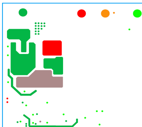
FIGURE 20. ETCH - LAYER 2
