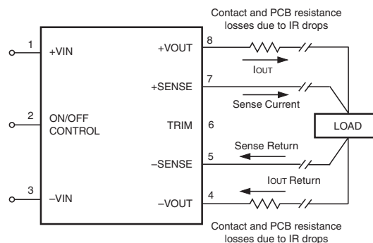
Figure 4. Remote Sense Circuit Configuration
