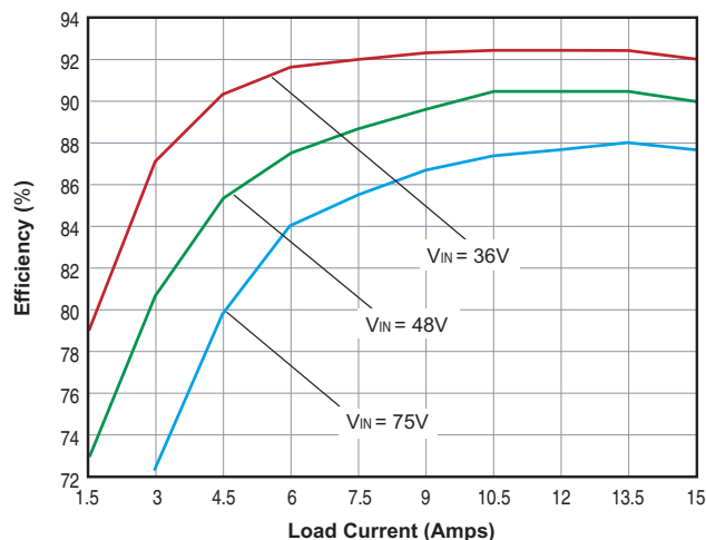
ULQ-2.5/15-D48 Efficiency vs. Line Voltage and Load Current
