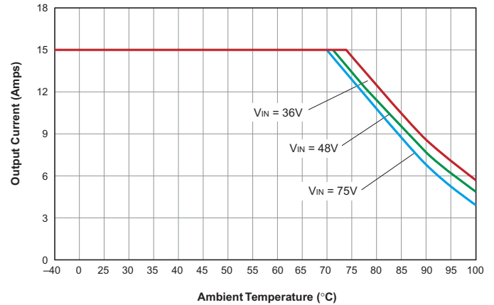
Output Current vs. Ambient Temperature (No air flow)
