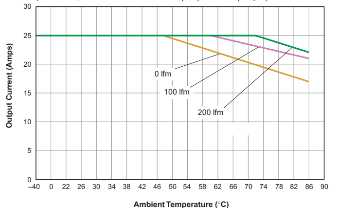
Output Current vs. Ambient Temperature ( V_{IN} = 48V , air flow direction from Input pin to Output pin)
