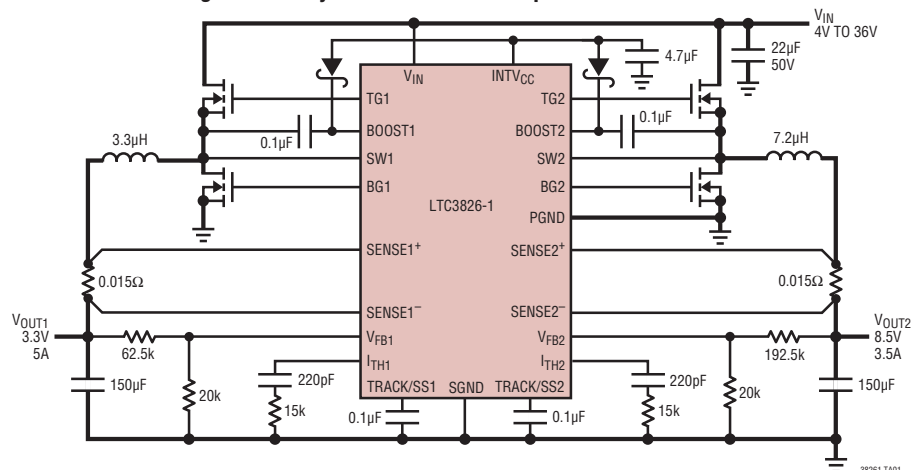
High Efficiency Dual 8.5V/3.3V Step-Down Converter
