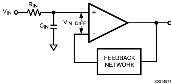
FIGURE 11. Alternative Sensor Impedance Circuit
