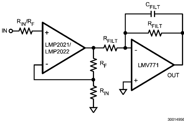
FIGURE 4. Enhanced Filter to Further Reduce Noise at Higher Gains
