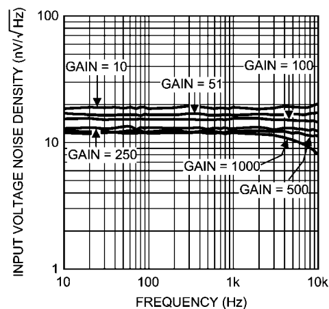
FIGURE 2. Input Voltage Noise Density with no 1/f
