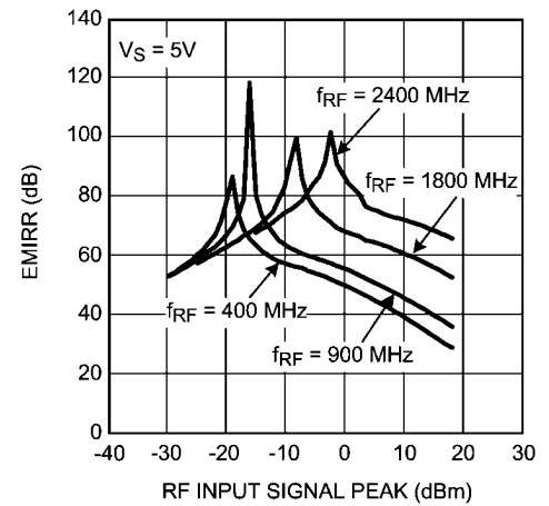
EMIRR vs. Input Power
