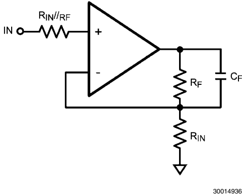
FIGURE 3. Noise Reducing Filter for Lower Gains
