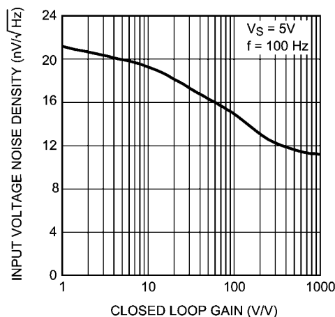
FIGURE 1. Input Voltage Noise Density decreases with Gain
