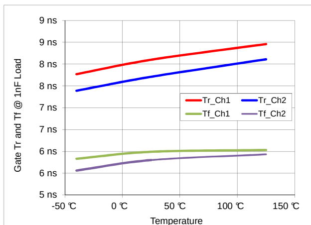
Figure 16: Gate Output Tr and Tf time @ 1nF Load vs. Temperature
