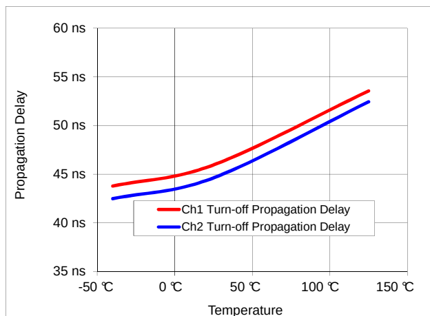
Figure 14: Turn-off Propagation Delay vs. Temperature
