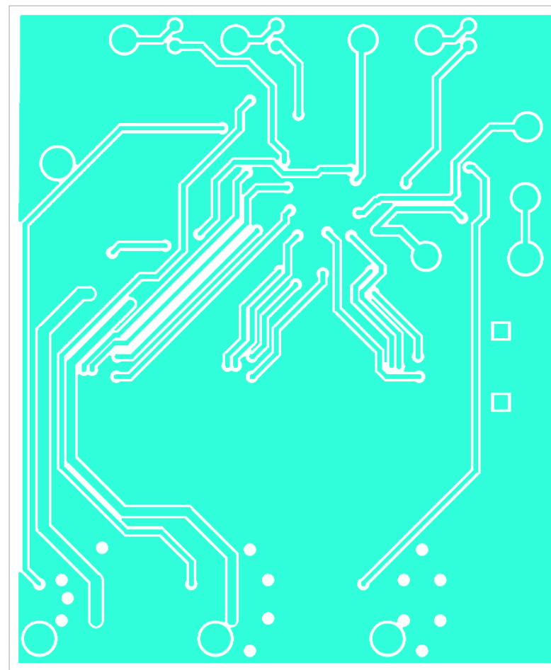
FIGURE 18. THIRD LAYER
