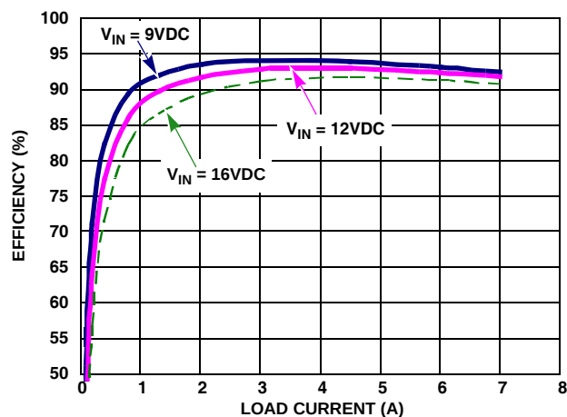
FIGURE 6. PWM2 EFFICIENCY vs LOAD ( V_O = 3.3V )
