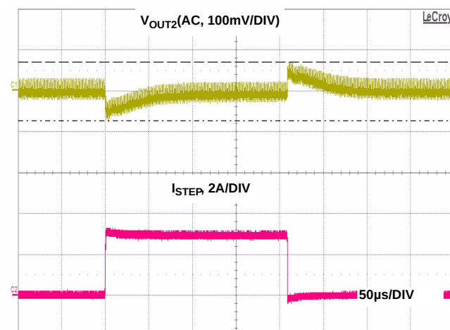
FIGURE 12. PWM2 LOAD TRANSIENT RESPONSE (LOAD STEP FROM 1.5A TO 4.5A)
