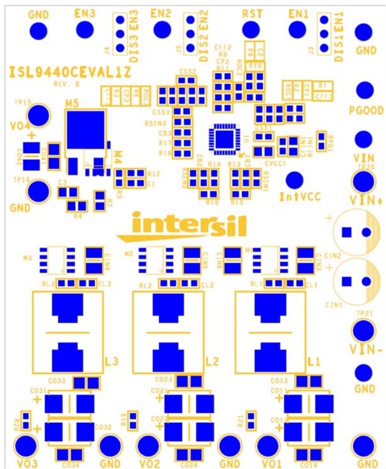
FIGURE 15. TOP COMPONENTS
