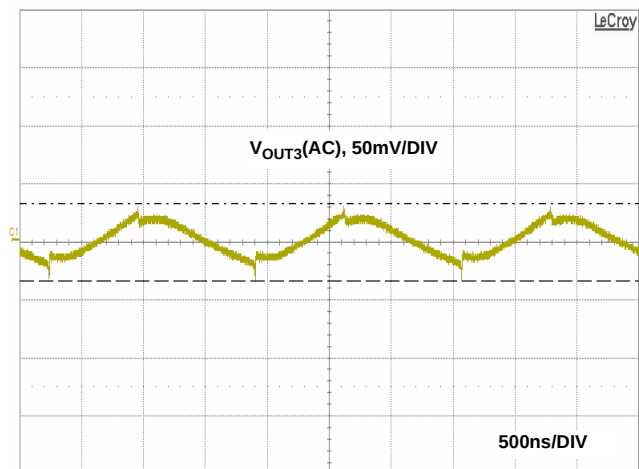
FIGURE 10. PWM3 OUTPUT RIPPLE UNDER MAX LOAD ( V_{IN} = 12V , I_{O1} = I_{O2} = 6A , I_{O3} = 4A , FULL BANDWIDTH)
