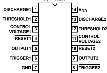
ICM7556 (14 LD PDIP) TOP VIEW
