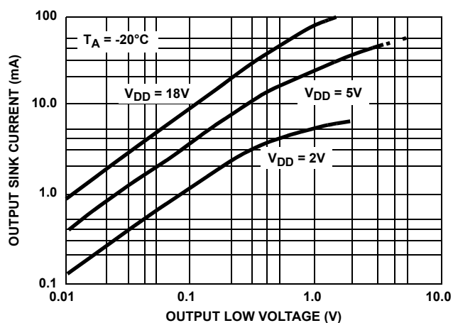
FIGURE 10. OUTPUT SINK CURRENT vs OUTPUT VOLTAGE
