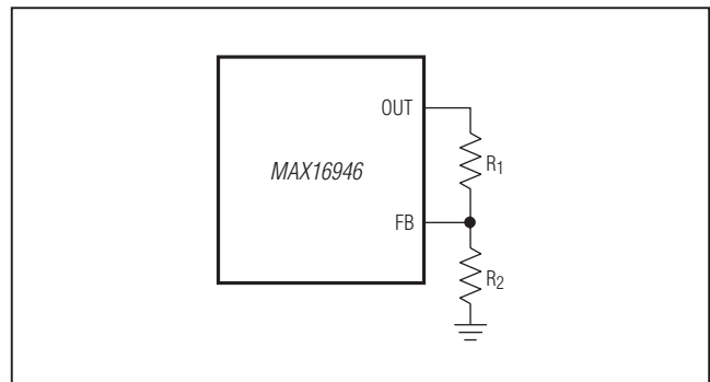
Figure 7. Adjustable Output-Voltage Selection
