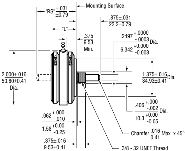
Model 5611 Bushing Mount with Sleeve Bearing
