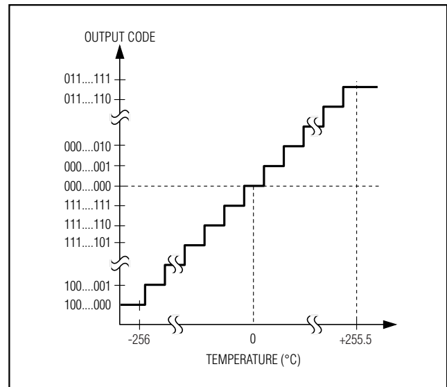
Figure 5. Temperature Transfer Function
