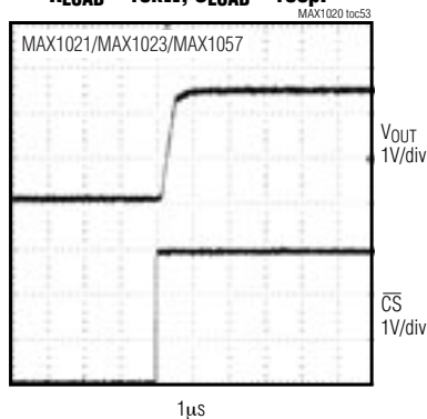
DYNAMIC RESPONSE RISE TIME R_{LOAD} = 10k\Omega , C_{LOAD} = 100pF
