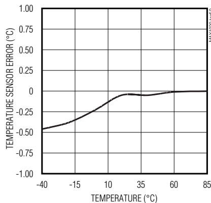
TEMPERATURE SENSOR ERROR vs. TEMPERATURE
