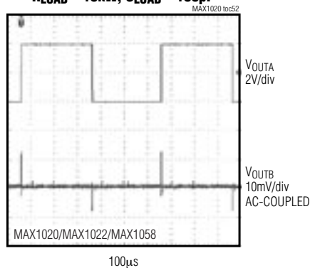
DAC-TO-DAC CROSSTALK R_{LOAD} = 10k\Omega , C_{LOAD} = 100pF
