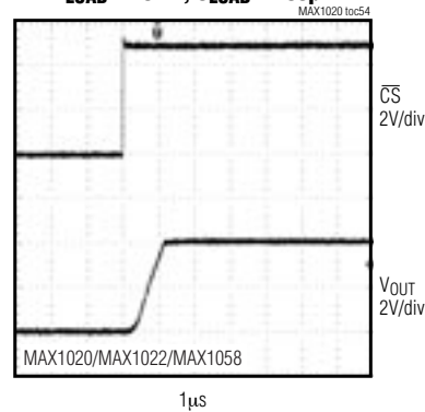
DYNAMIC RESPONSE RISE TIME R_{LOAD} = 10k\Omega , C_{LOAD} = 100pF
