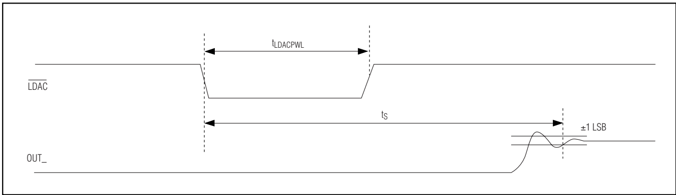
Figure 14. \overline{\text{LDAC}} Functionality
