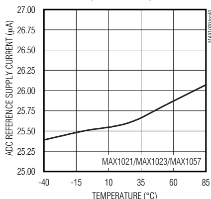
ADC REFERENCE SUPPLY CURRENT vs. TEMPERATURE
