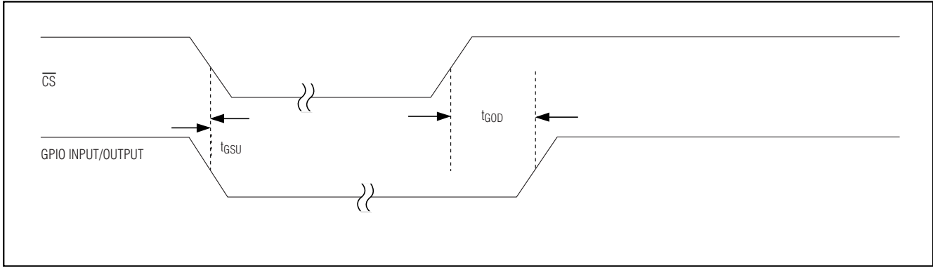
Figure 13. GPIO Timing
