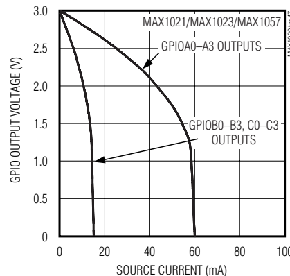
GPIO OUTPUT VOLTAGE vs. SOURCE CURRENT
