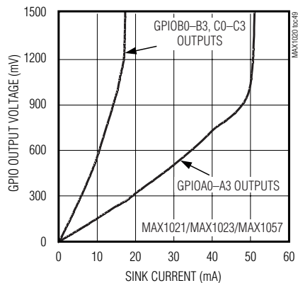
GPIO OUTPUT VOLTAGE vs. SINK CURRENT
