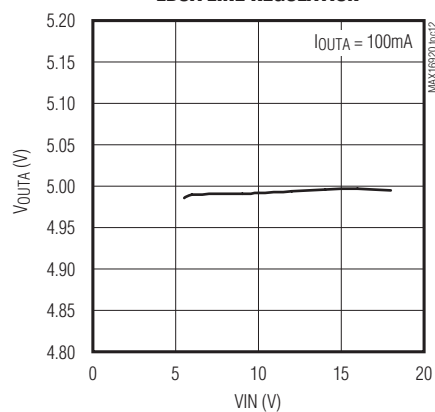
LDOA LINE REGULATION
