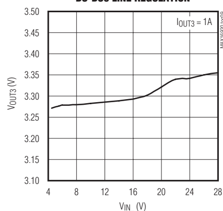
DC-DC3 LINE REGULATION
