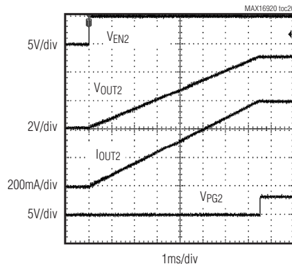
DC-DC2 STARTUP INTO FULL LOAD
