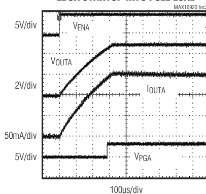
LDOA STARTUP INTO FULL LOAD
