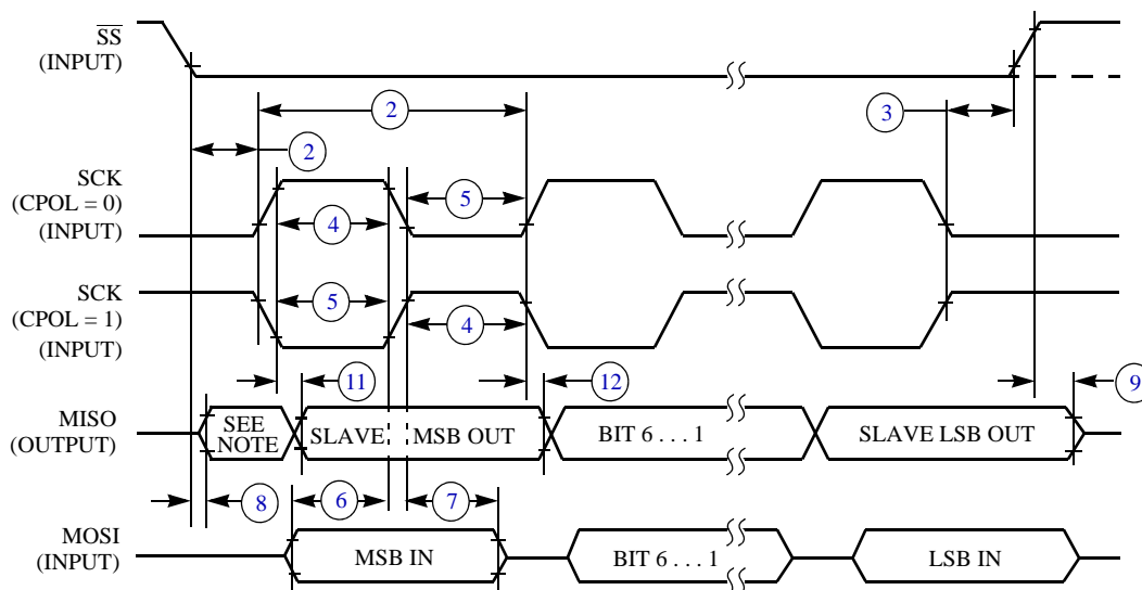
Figure 21. SPI Slave Timing (CPHA = 0)
