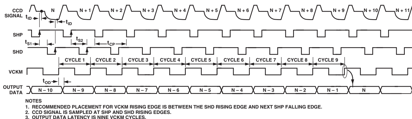
Figure 40. Pipeline Latency
