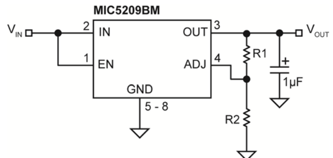
Figure 3. Low-Noise Adjustable Voltage Regulator
