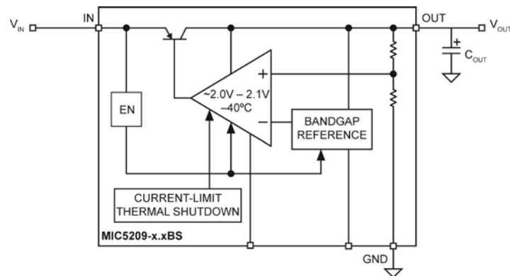
Low-Noise Fixed Regulator (SOT-223 Version Only)
