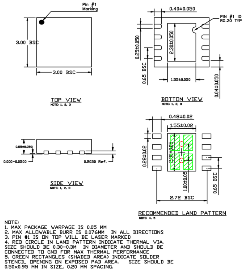
8-Pin 3mm x 3mm DFN (ML)
