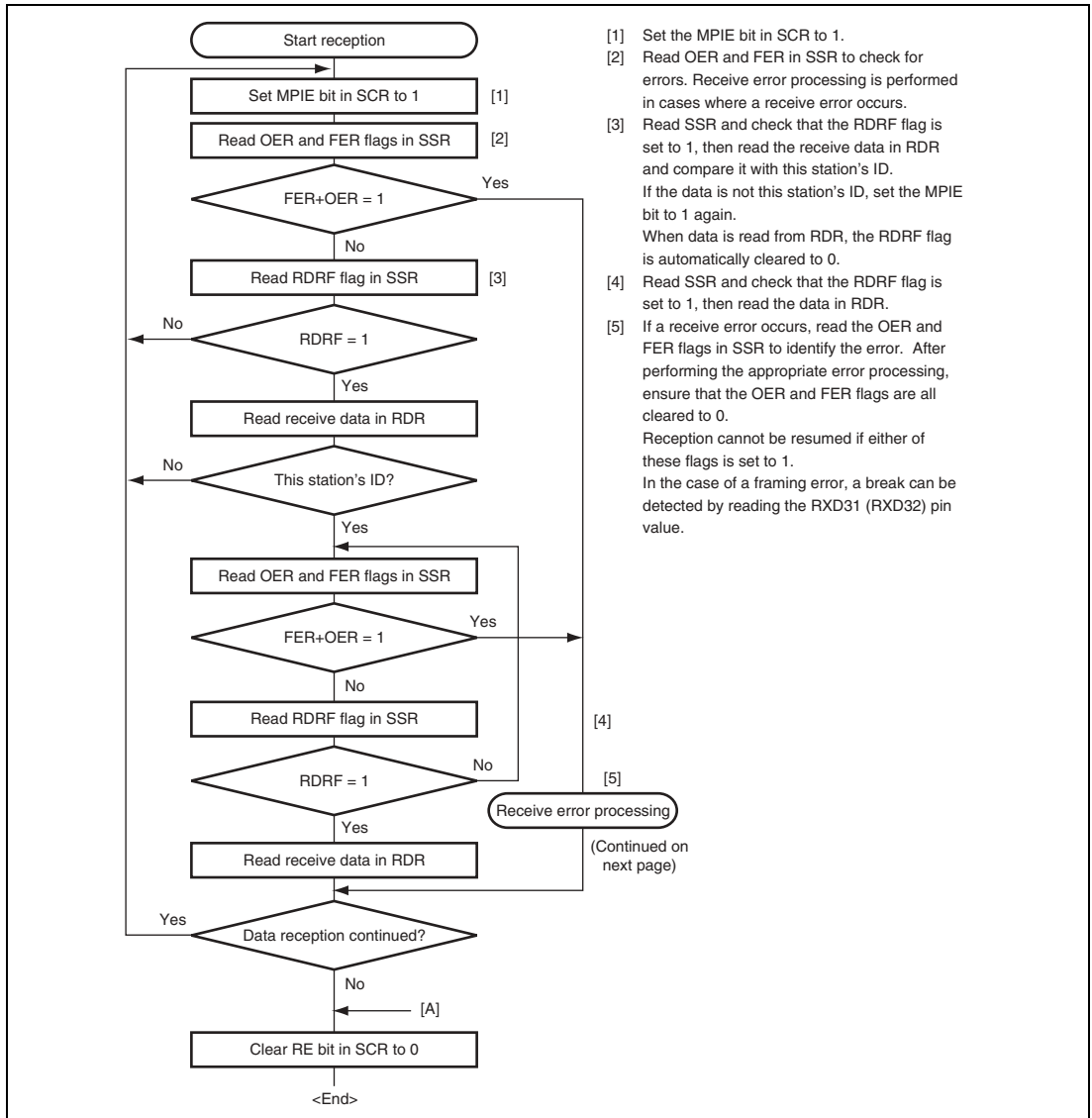
Figure 15.17 Sample Multiprocessor Serial Reception Flowchart (1)
