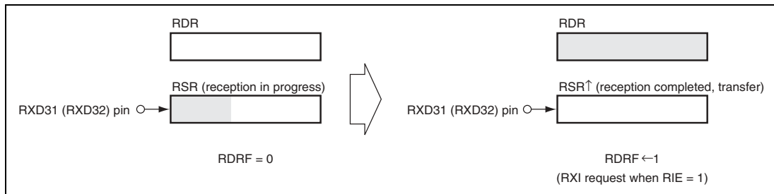
Figure 15.21 (a) RDRF Setting and RXI Interrupt
