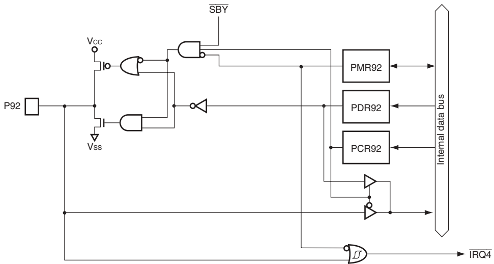
Figure B.8 (a) Port 9 Block Diagram (P93)
