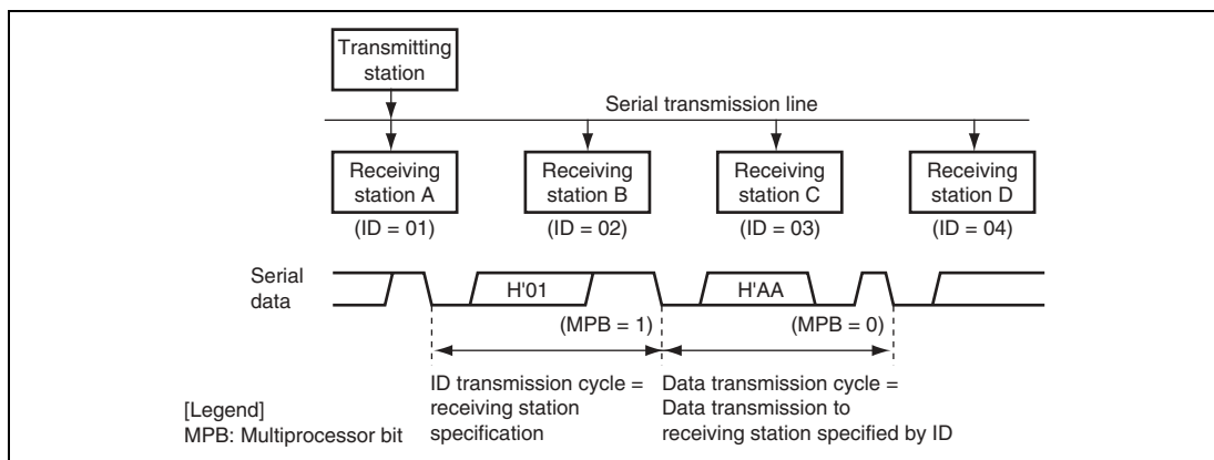
Figure 15.15 Example of Communication Using Multiprocessor Format (Transmission of Data H'AA to Receiving Station A)
