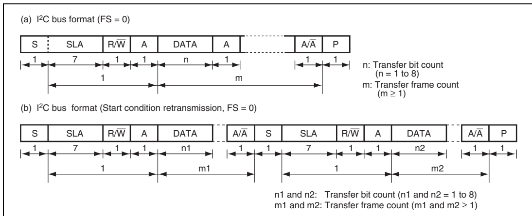
Figure 21.3 I 2 C Bus Formats
