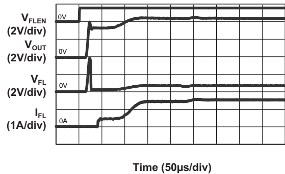
Flash Turn On Characteristic
