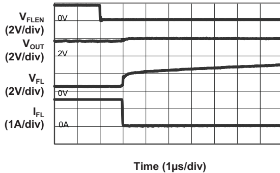
Flash Turn Off Characteristic
