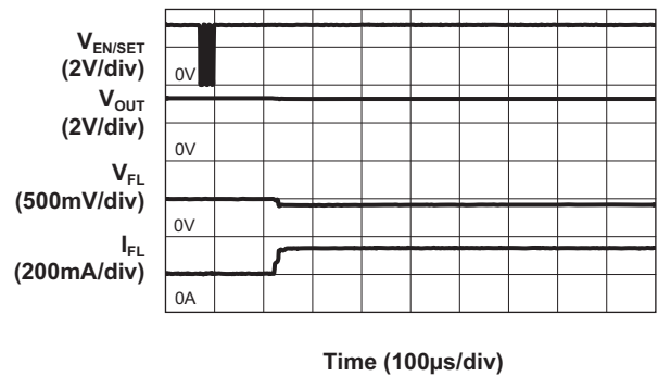
Movie Mode Transition Characteristic
