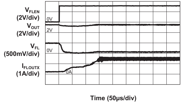
Movie Mode to Flash Turn On Characteristic
