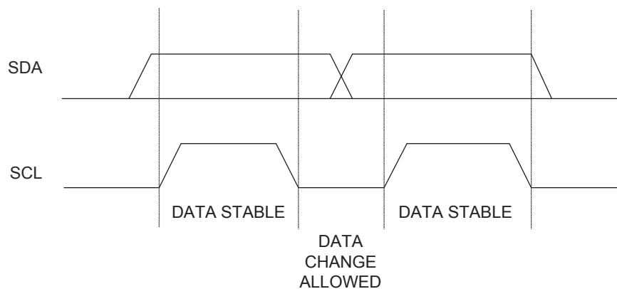
Figure 5-3. Data Validity
