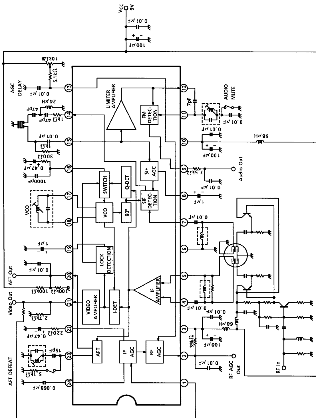
APPLICATION CIRCUIT 1 (SPLIT CARRIER)
