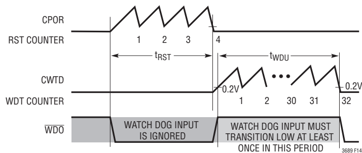
(14c) \overline{W}/T = Low. Restart Sequence After a Timing Fault
