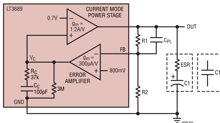
Figure 3. Model for the Loop Response
