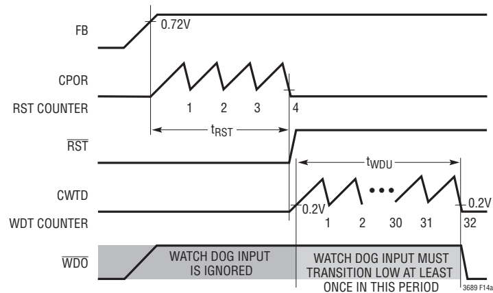
(14a) \overline{W}/T = High. The First Valid Negative Edge on WDI Must Occur Before the Watchdog Timer Expires
