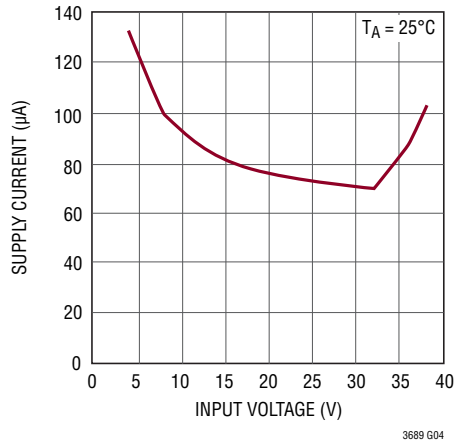
No-Load Supply Current vs V_{IN}
