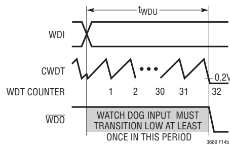
(14b) \overline{W}/T = High. Subsequent Edges Must Occur Before the Timer Expires
