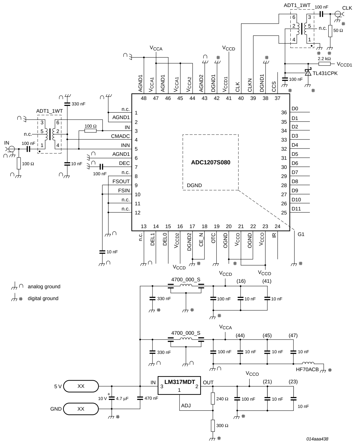
Fig 10. Application diagram
