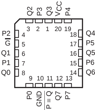
54ACT11521 . . . FK PACKAGE (TOP VIEW)
