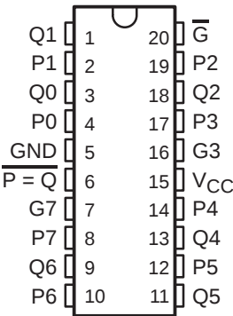
54ACT11521 . . . J PACKAGE 74ACT11521 . . . DB, DW OR N PACKAGE (TOP VIEW)
