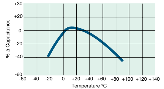
Temperature Coefficient
