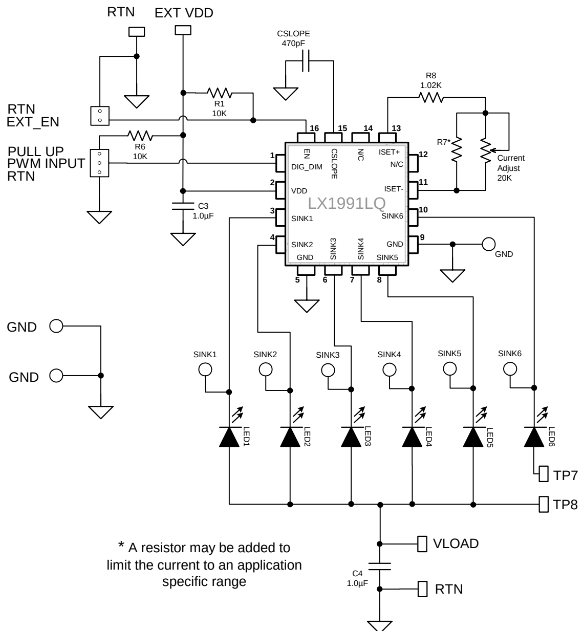
Figure 2 – Schematic
