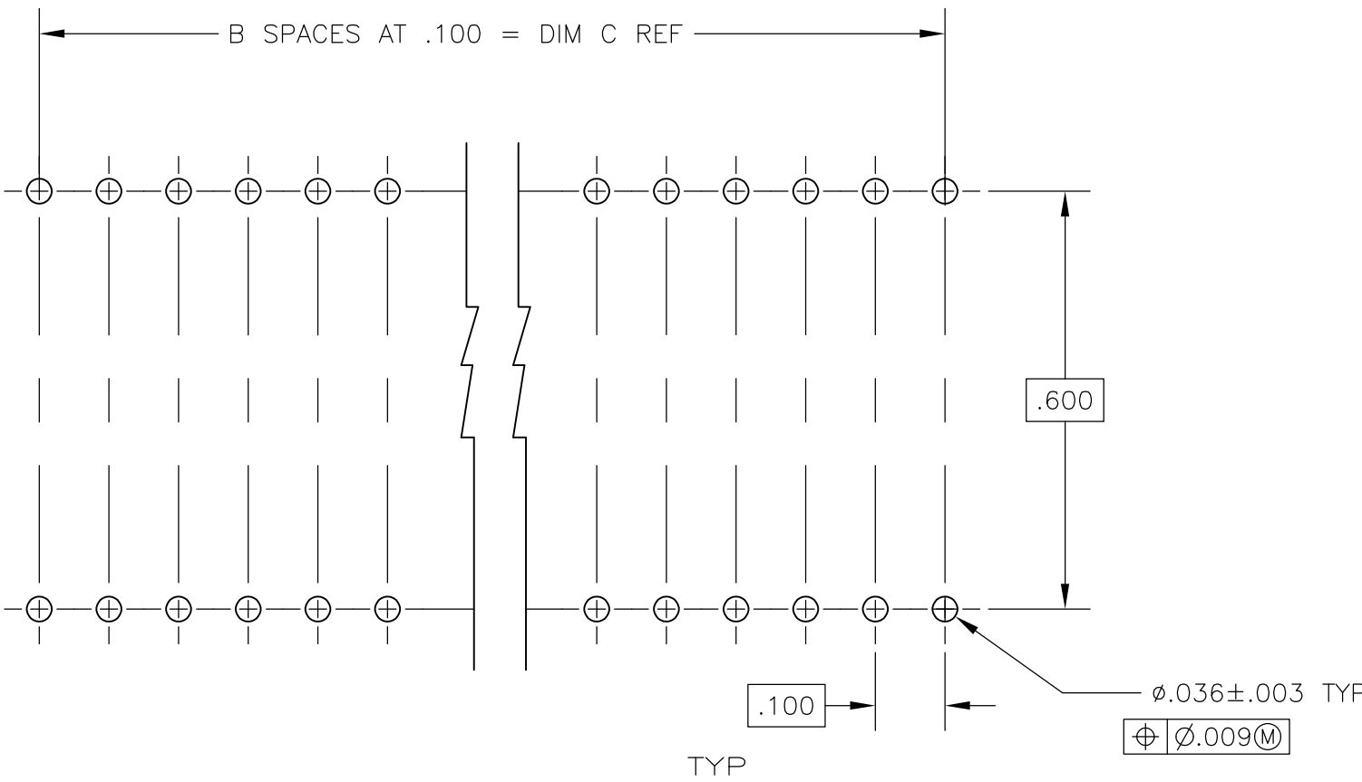
RECOMMENDED MOUNTING HOLE PATTERN SCALE 4:1
