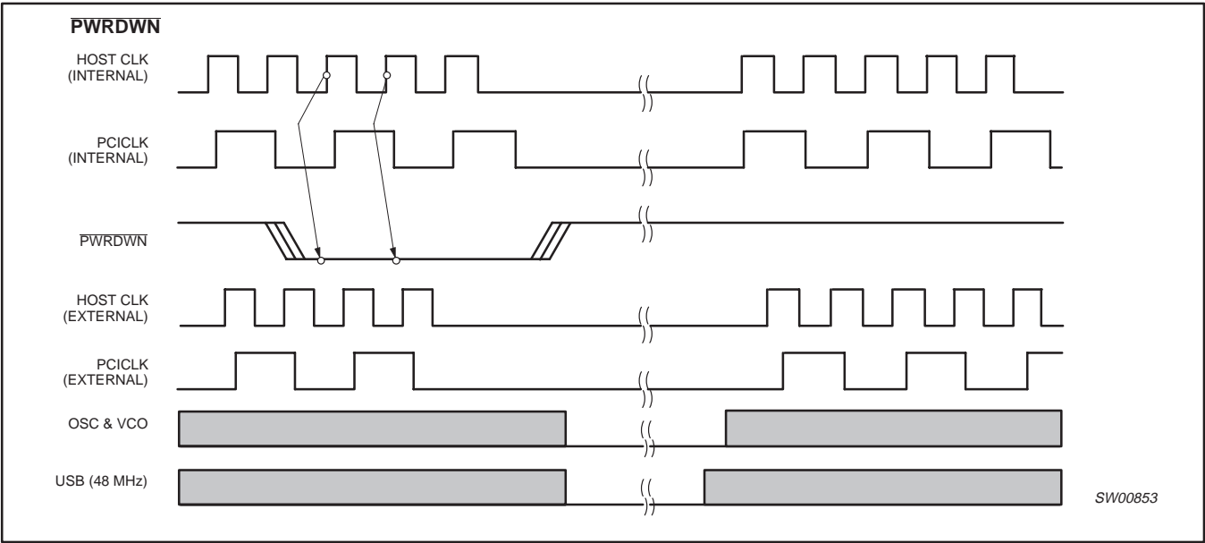
Figure 5. Power management
