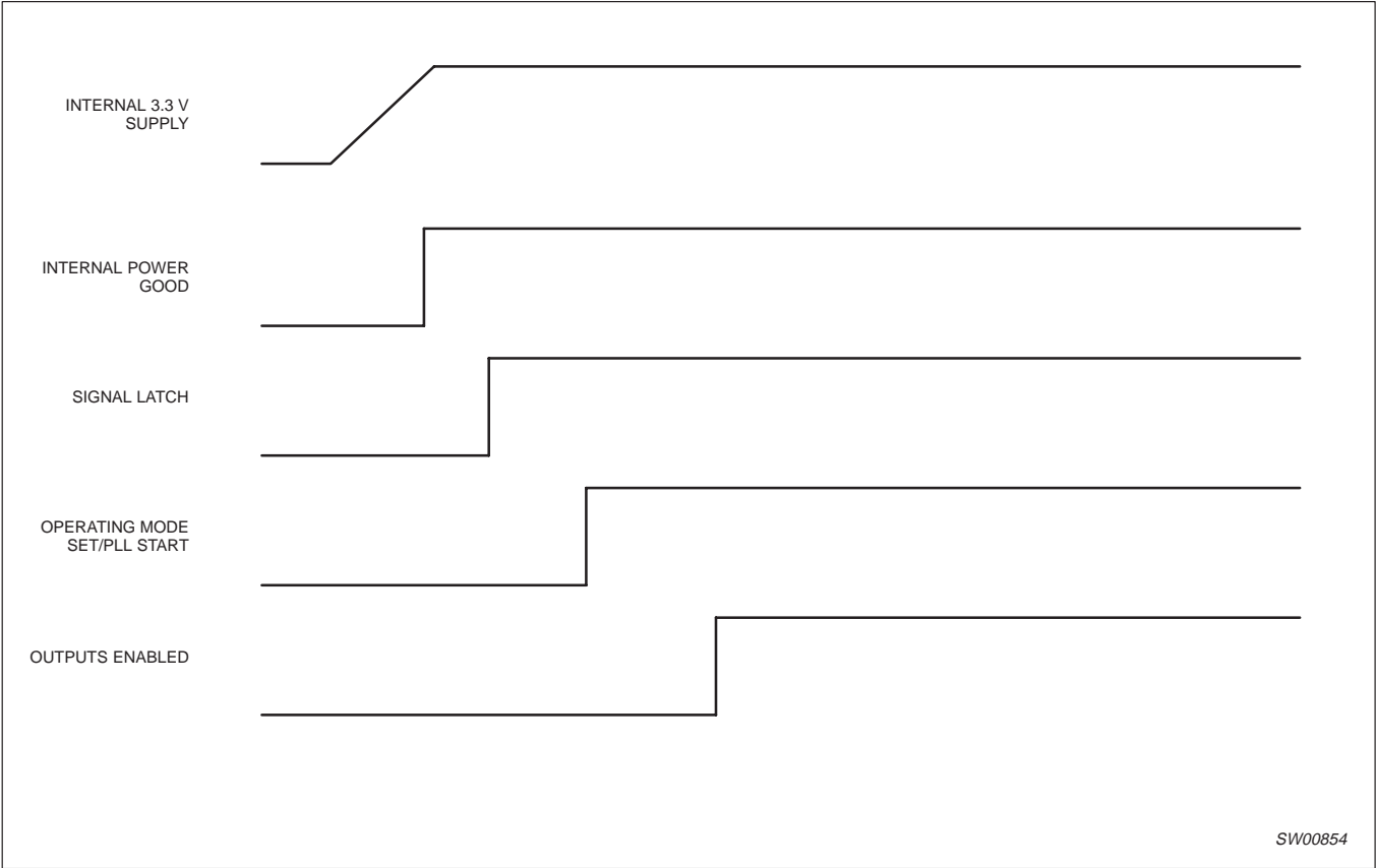
Figure 6. Power-up sequence
