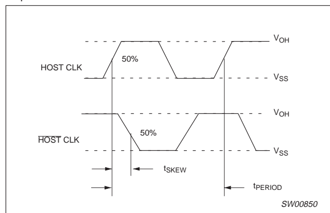
Figure 1. Host clock
