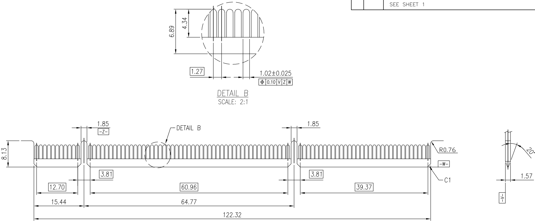
RECOMMENDED MATING COMPONENT BOARD (3.3V) Tolerance: ±0.05
