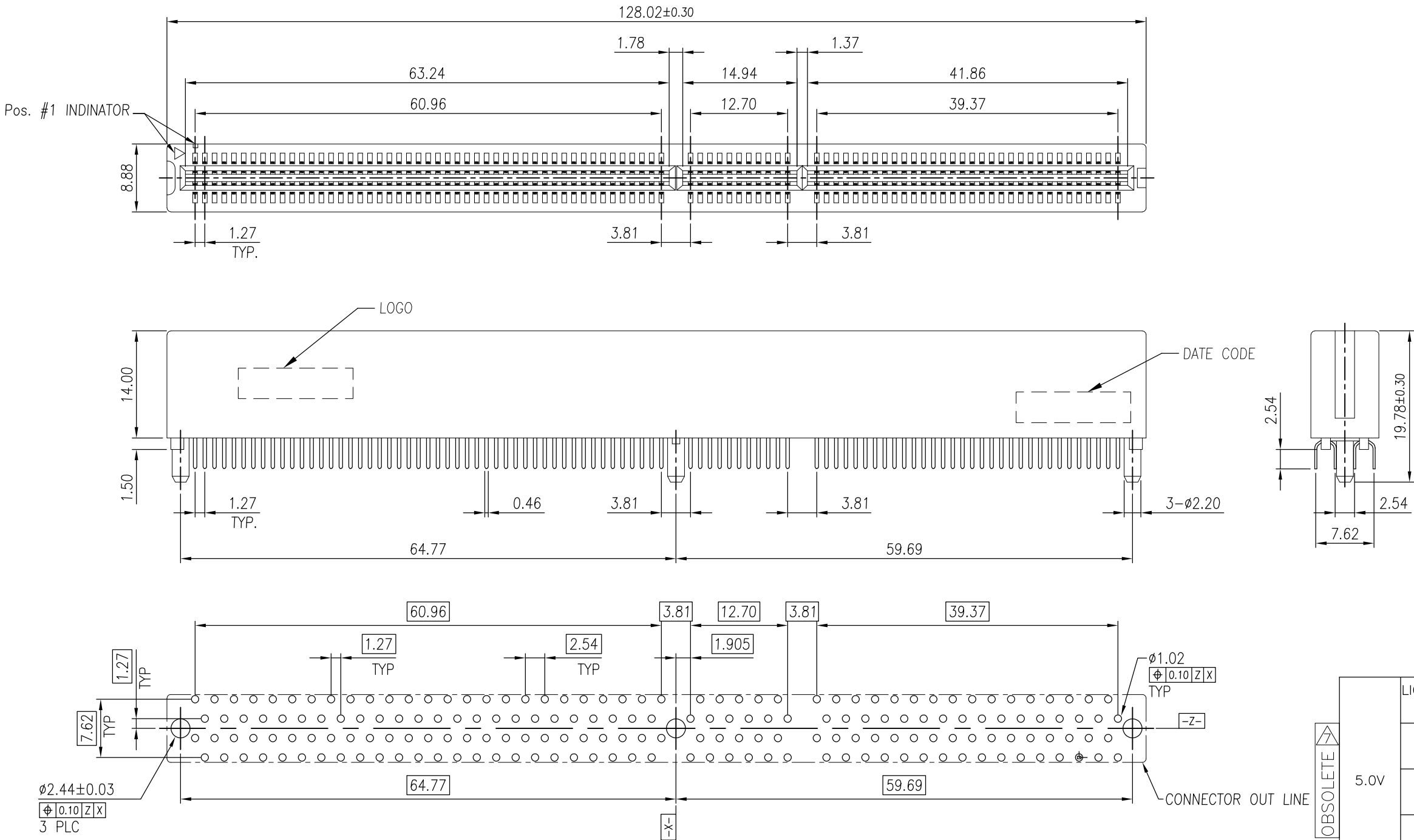
RECOMMENDED PCB LAYOUT (TOP VIEW) TOLERANCE : ±0.05
