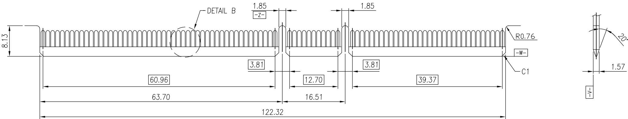
RECOMMENDED MATING COMPONENT BOARD (5.0V) Tolerance: ±0.05
