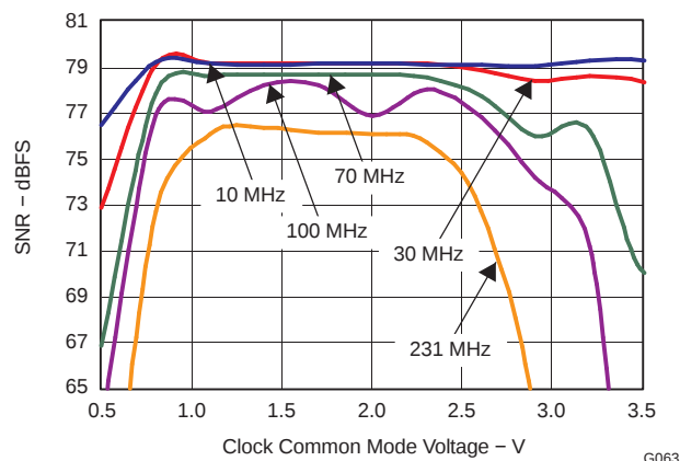
Figure 73. SNR versus Clock Common Mode
