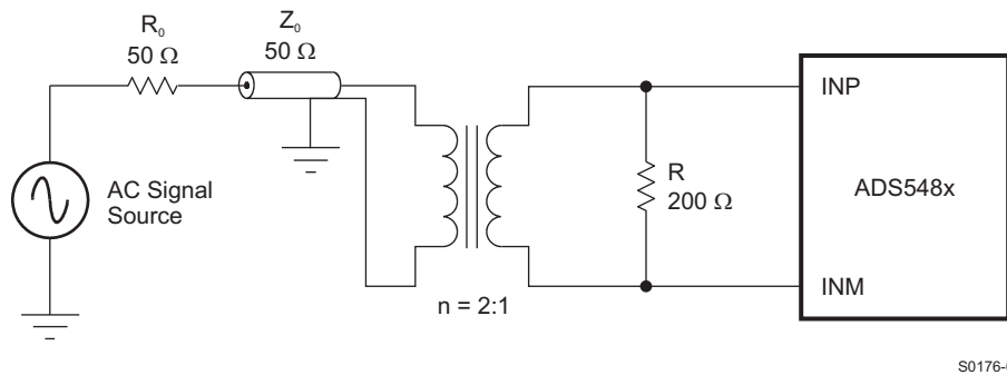
Figure 61. Converting a Single-Ended Input to a Differential Signal Using an RF Transformer
