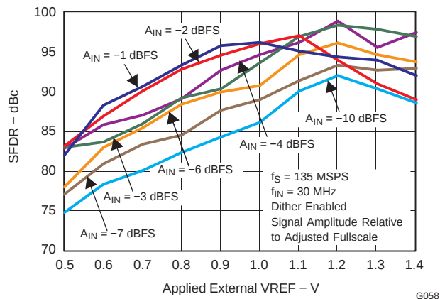
Figure 63. SFDR versus External VREF and A_{IN}
