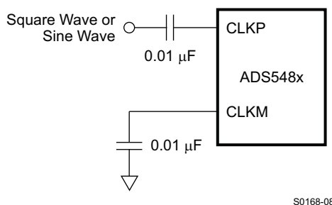
Figure 68. Single-Ended Clock
