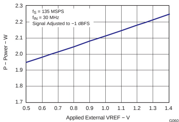
Figure 65. Total Power Consumption versus External VREF
