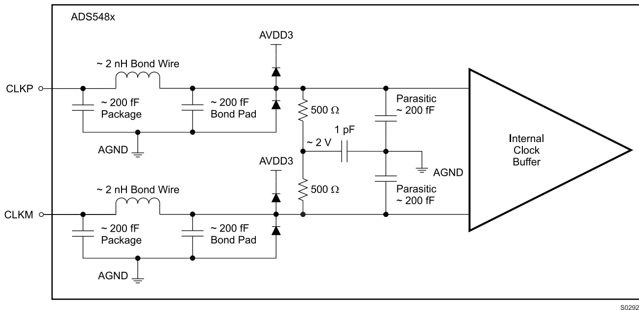
Figure 67. Clock Input Circuit
