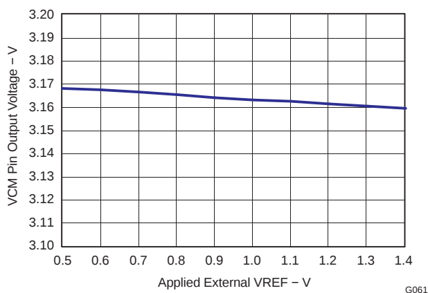
Figure 66. VCM Pin Output versus External VREF
