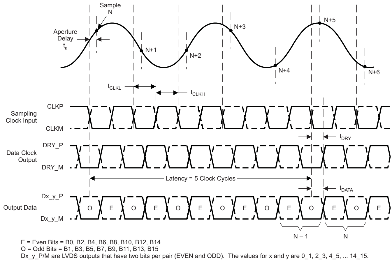
Figure 1. Timing Diagram
