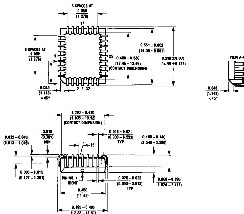
32-Lead PLCC Package Order Number NMC27C512AV
