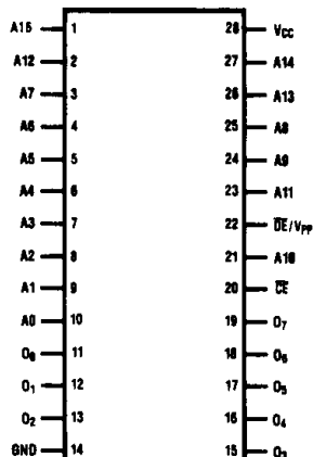
NMC27C512AN Dual-In-Line Package
