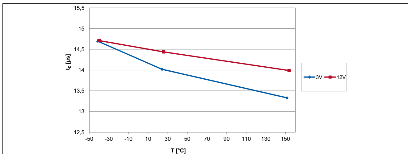
Figure 6-2 Signal Delay Time of the TLV4961-3M over Temperature
