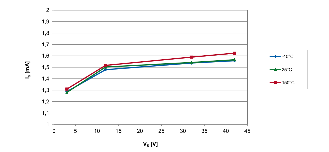
Figure 6-4 Supply Current of the TLV4961-3M over Supply Voltage
