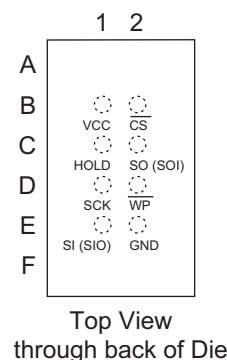
Figure 2-3. 8-ball dBGa (Top View)
