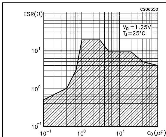
Figure 25. Stability
