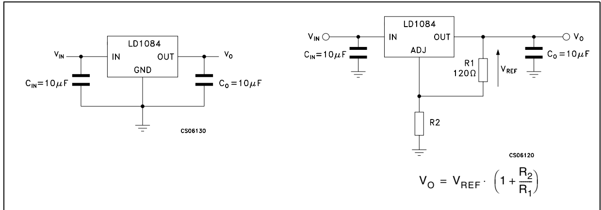
Figure 2. Application circuit
