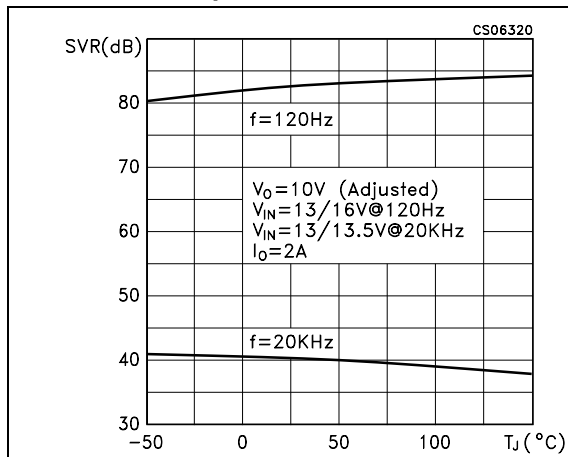
Figure 21. Supply voltage rejection vs temperature
