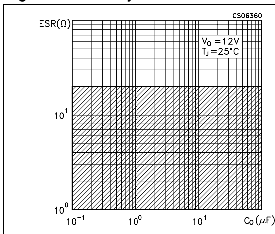
Figure 25. Stability
