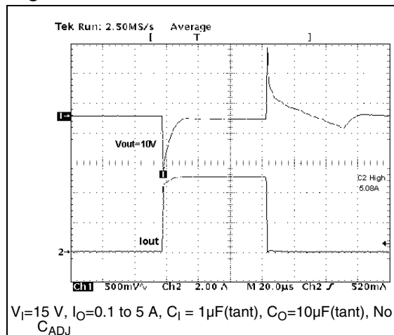
Figure 31. Load Transient
