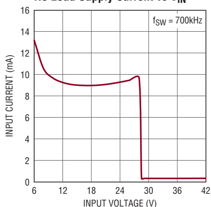
No Load Supply Current vs V_{IN}
