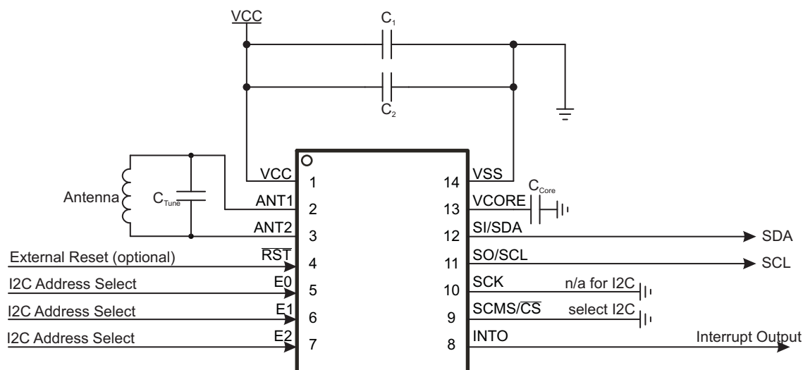
Figure 3-2. Example Application Diagram (I 2 C Operation)
