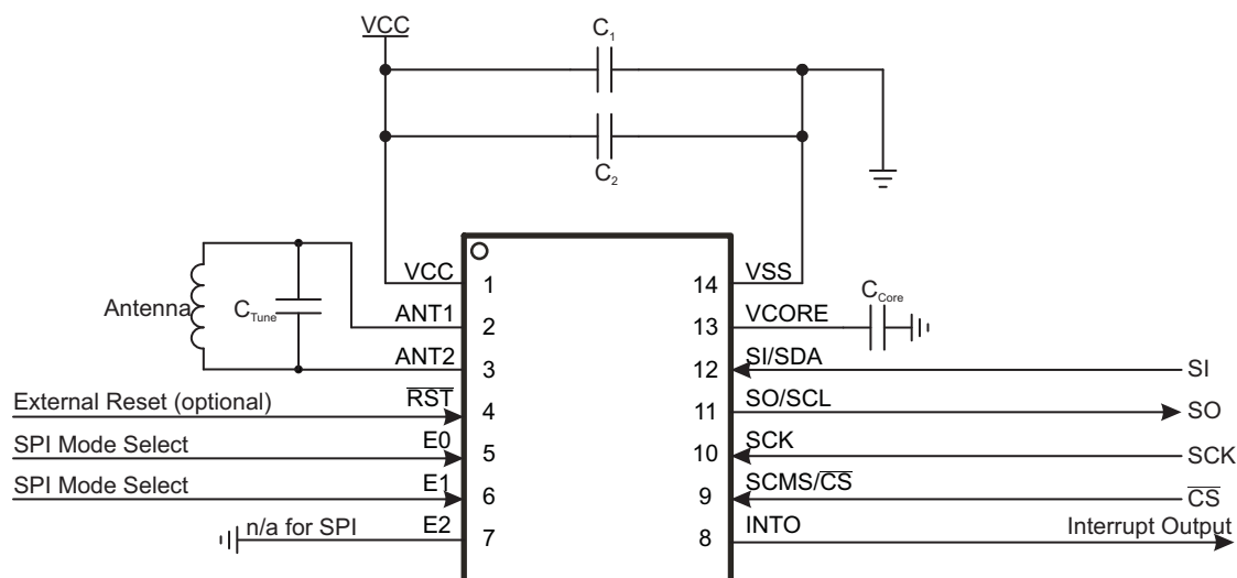
Figure 3-3. Example Application Diagram (SPI Operation)
