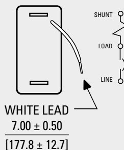
Shunt Trip Single Pole
