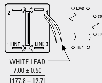
Two Pole ( 1 pole relay)
