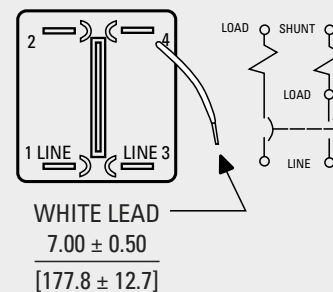
Two Pole ( 1 pole shunt)
