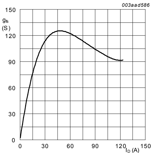
Fig. 8. Forward transconductance as a function of drain current; typical values T_j = 25^\circ\text{C}; V_{DS} = 15\text{V}
