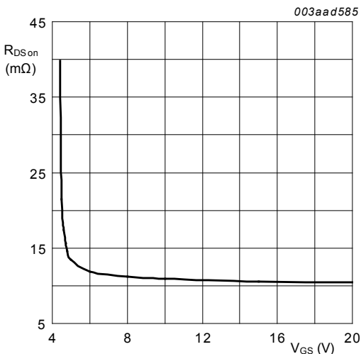
Fig. 7. Drain-source on-state resistance as a function of gate-source voltage; typical values T_j = 25^\circ\text{C}
