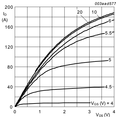
Fig. 5. Output characteristics: drain current as a function of drain-source voltage; typical values T_j = 25^\circ\text{C}
