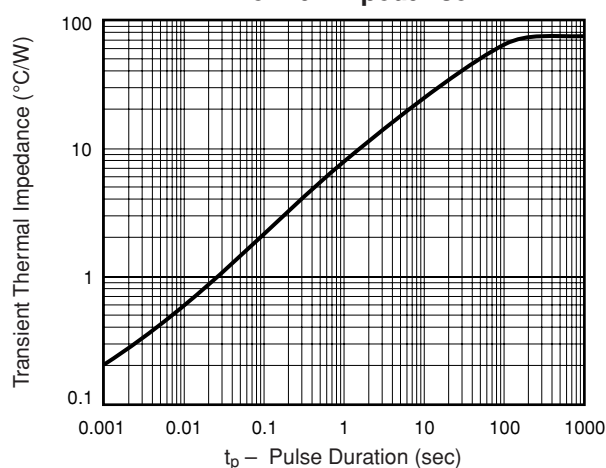
Fig. 12 – Typical Transient Thermal Impedance
