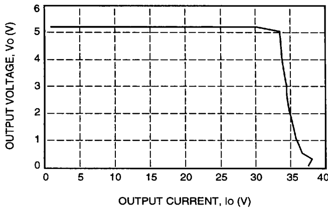
Figure 2. Typical FE150N Output Characteristics at Room Temperature and 48 V Input
