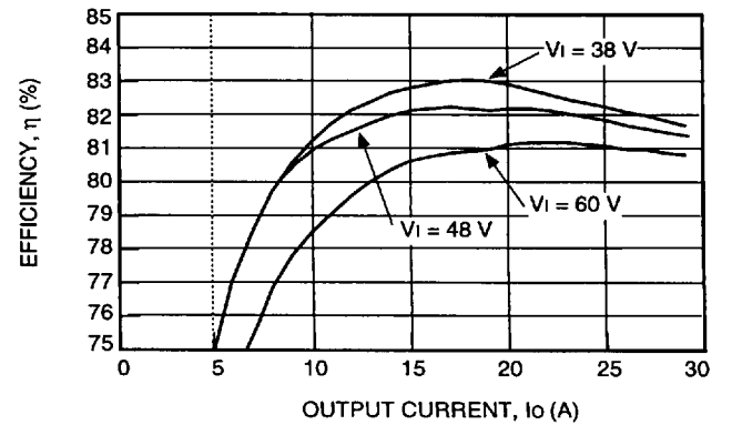
Figure 4. Typical FE150N Efficiency vs. Output Current at Room Temperature
