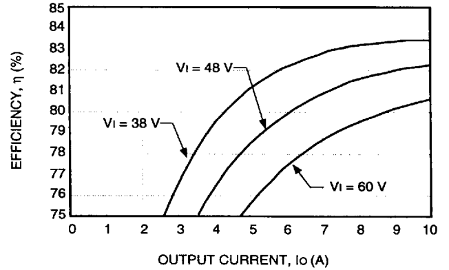
Figure 3. Typical FE050N Efficiency vs. Output Current at Room Temperature
