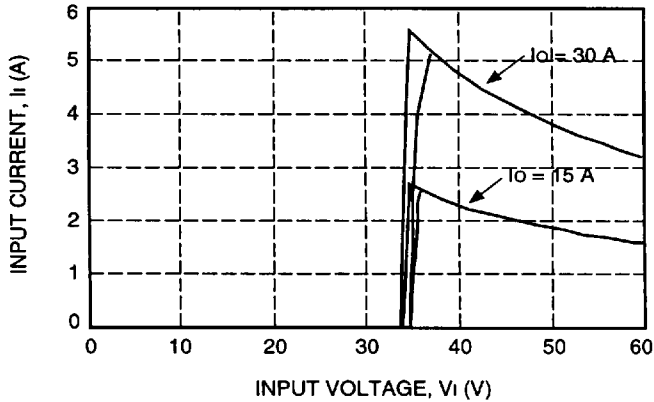
Figure 1. Typical FE150N Input Characteristics at Room Temperature
